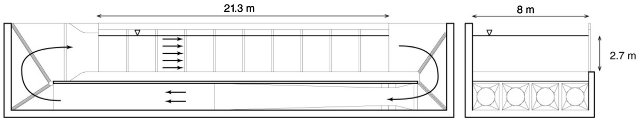
Fig. 1. The North Sea Centre Flume Tank in Hirtshals, Denmark, with an experimental section measuring 21.3 m long, 2.7 m deep and 8 m wide.
